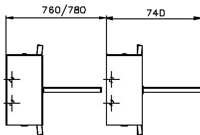
Floor anchor position (drilled during installation).
