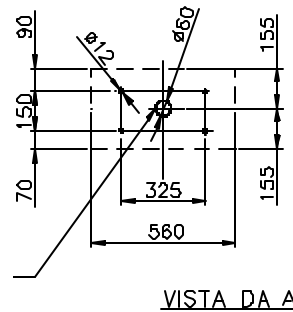
Cable entry
